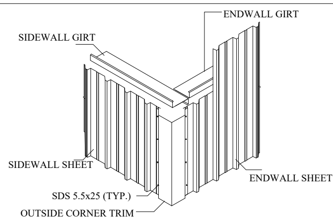
CORNER TRIM DETAIL (3-D)
