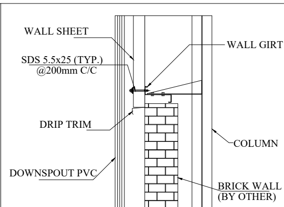
DRIP TRIM DETAIL
